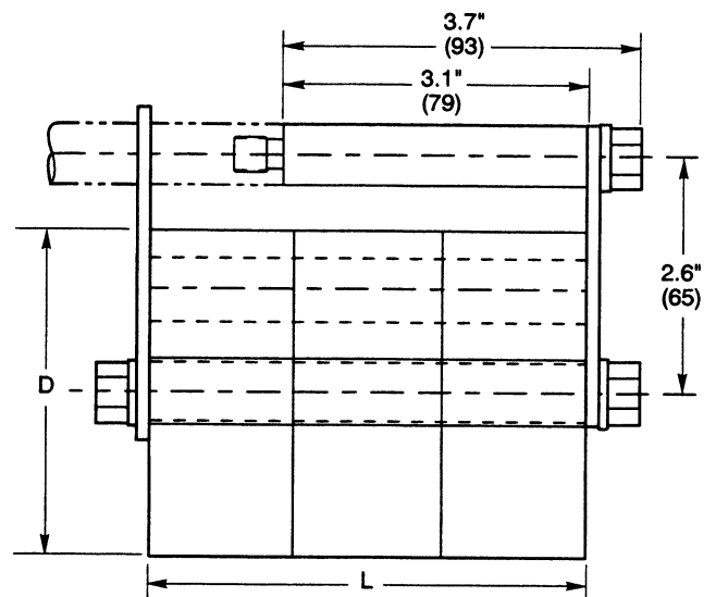
Weighted Horizontal Displacer, Extended Control, Multiple Disc's.
