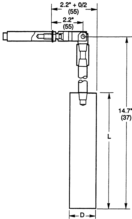
Standard Vertical Displacer, Solid, Extended Control.
