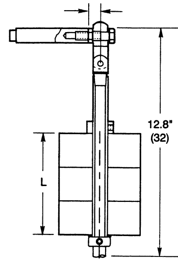
Vertical Displacer, Thru-hole, Extended Control, Multiple Discs.
