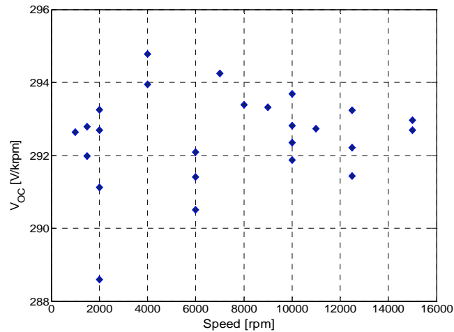
Fig 12. Measured Open Circuit Voltage
