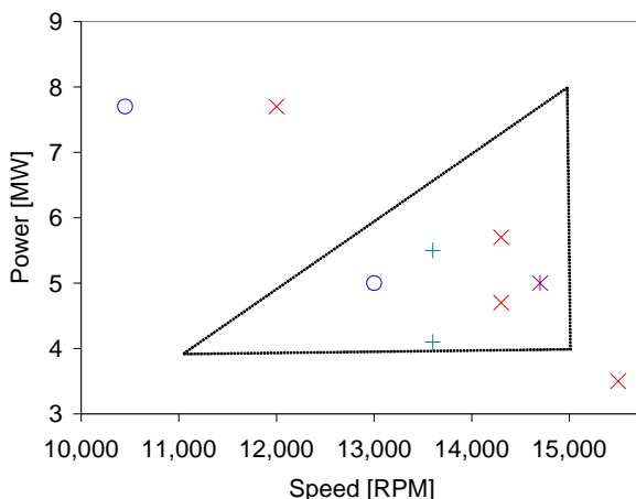
Fig 1. Gas Turbine Ratings from Various Manufacturers [11]
