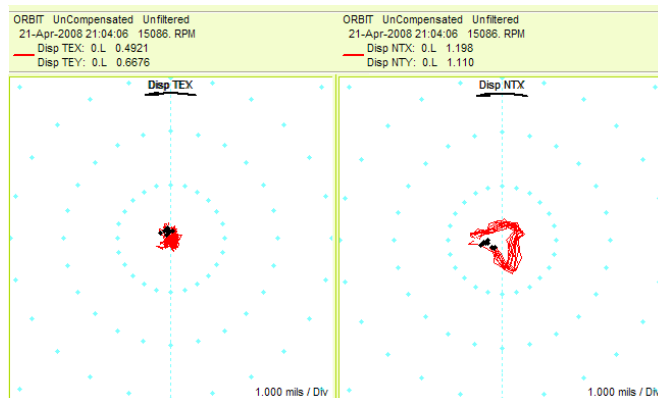
Fig 21. Drive End (left) and Non-Drive End (right) X-Y Orbit Plot at 15086 RPM
