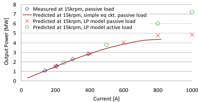
Fig 23. Predicted and Measured Output Power at 15 kRPM
