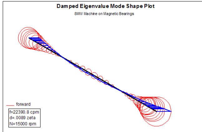
Fig 4. Mode Shape for the First Forward Bending Mode of Magnetic Bearing Configuration
