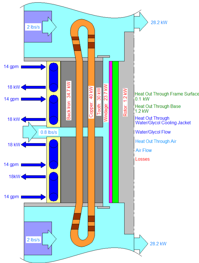
Fig 8. Machine Cross-Section Showing Cooling System
