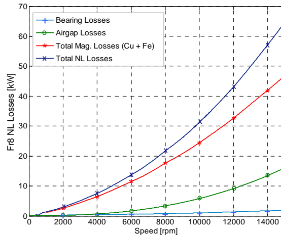
Fig 17. No-load Loss Segregation
