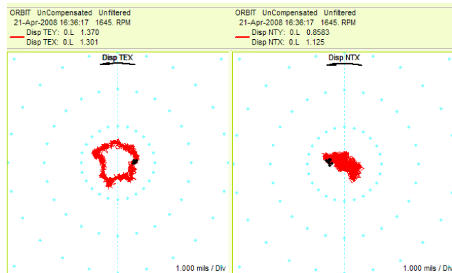
Fig 20. Drive End (left) and Non-Drive End (right) X-Y Orbit Plot at 1645 RPM
