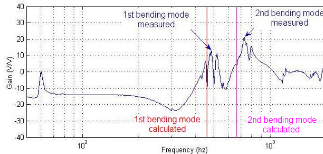
Fig 19. Rotor Impact Modal Test Results
