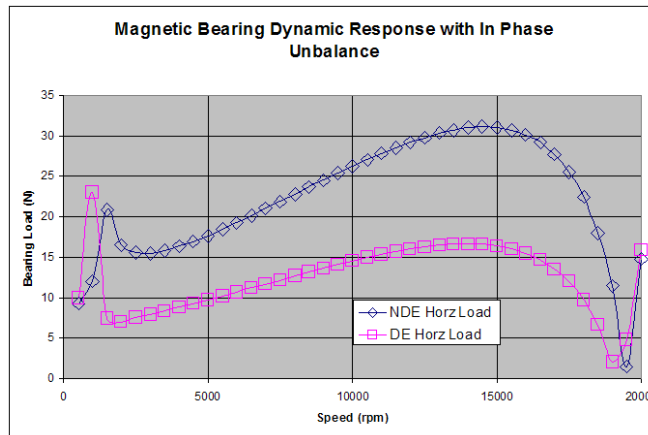
Fig 6. Bearing Load Response Plot For Magnetic Bearing Configuration
