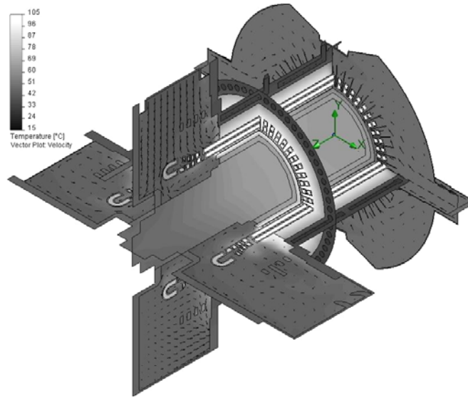
Fig 9. Solid Model Results from Computational Fluid Dynamic Analysis of Machine
