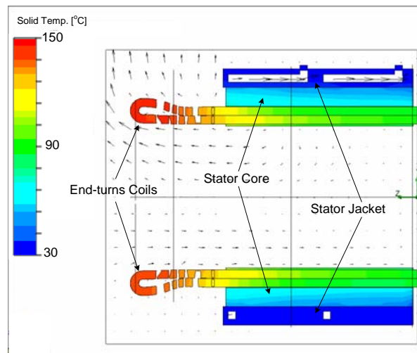
Fig 15. Stator Temperature Distribution (Longitudinal View)
