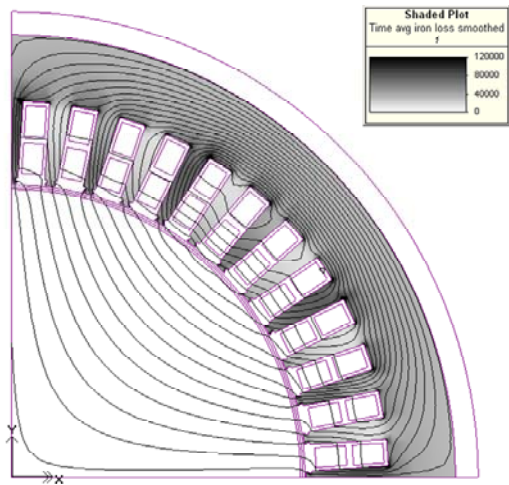
Fig 16. Iron Loss Distribution in the Stator from FEA during Stator-Only Testing
