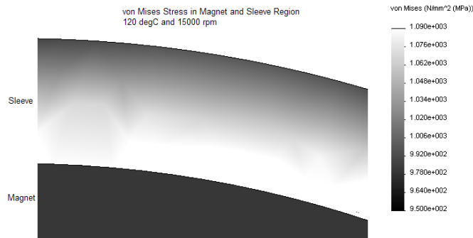
Fig 2. Von Mises Stress Distribution at 15kRPM and 120°C
