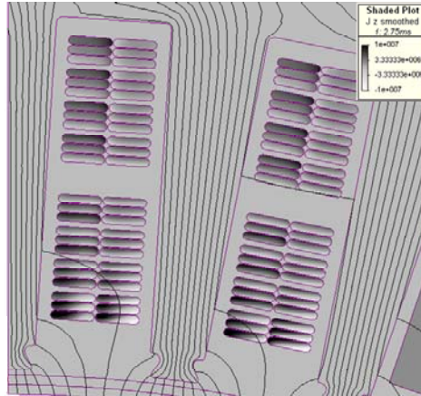
Fig 24. Current Density Distribution in the Stator Coils for the 3MW Load Generator Case at 500 Hz, 15 kRPM
