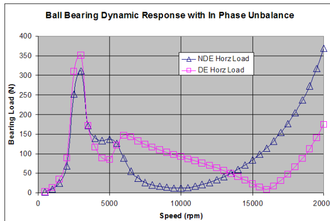
Fig 7. Bearing Load Response Plot For Ball Bearing Configuration
