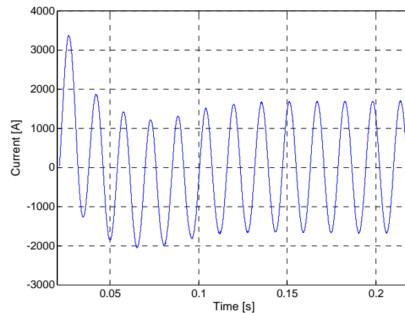
Fig 13. Measured Short Circuit Current
