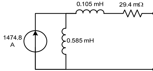
Fig 11. Simple Current-Driven per Phase Equivalent Circuit
