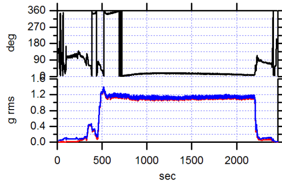
Fig 22. Drive End Vibration Bode Plot for a 40 Minute Test with a Max Rotor Speed of 15 kRPM from 500 sec to 2200 sec
