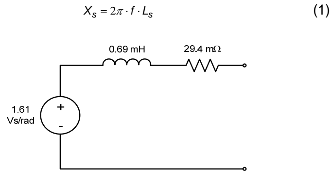
Fig 10. Simple Voltage Driven per Phase Equivalent Circuit
