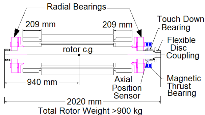
Fig 3. Magnetic Bearing and Rotor Layout
