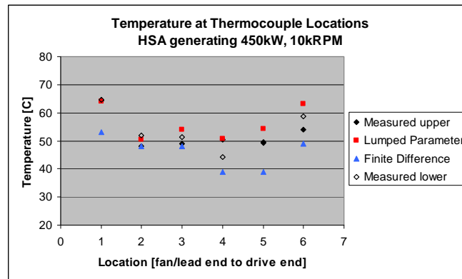
Fig. 14 Comparison Plot of Analytical Prediction and Test Data
